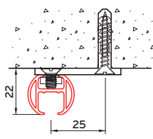
ceiling fixing with plate 5135
