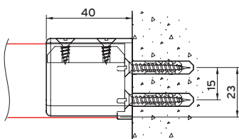
end fixing 4100 with support 4150
