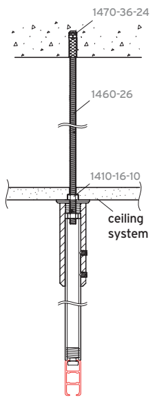
ceiling fixing with hanger 4155 and threaded rod through suspended ceiling tiles
