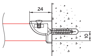
end fixing 4200 with support 4249
