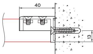
end fixing 5100 with support 5150
