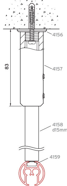
ceiling fixing with suspension hanger 4155
