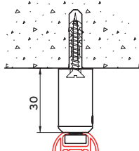
ceiling fixing with mini suspension hanger 4254
