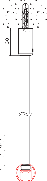
ceiling fixing with suspension hanger 4255
